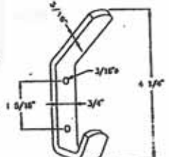
Coat Hook Zinc or Chrome part no. 209
