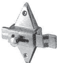
SLIDE BOLT/LATCH 1-7/8" Bet. Screws 5/16" Bars to Door Clearance Part No. 90T160
