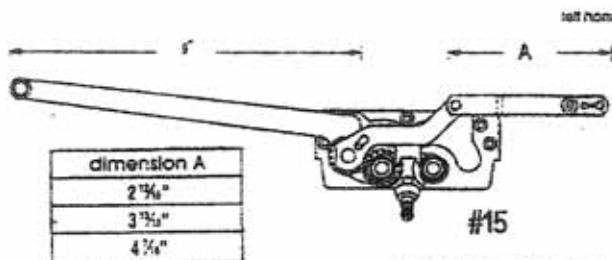
TRUTH ENTRY GARD
