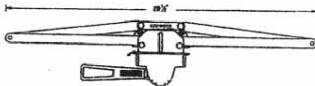
Lever lock #336-18G TRUTH
