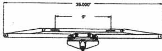
ROTO GEAR AWNING (Dual Pull) Part No. RO1114 TRUTH
